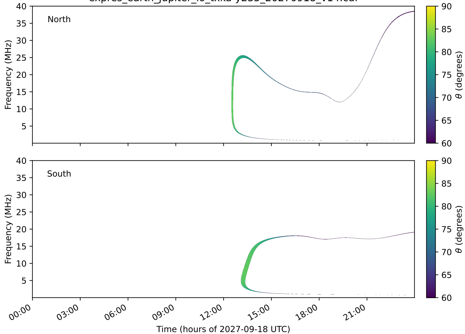
expres_earth_jupiter_io_txka-y235_20270918_v14.cdf
