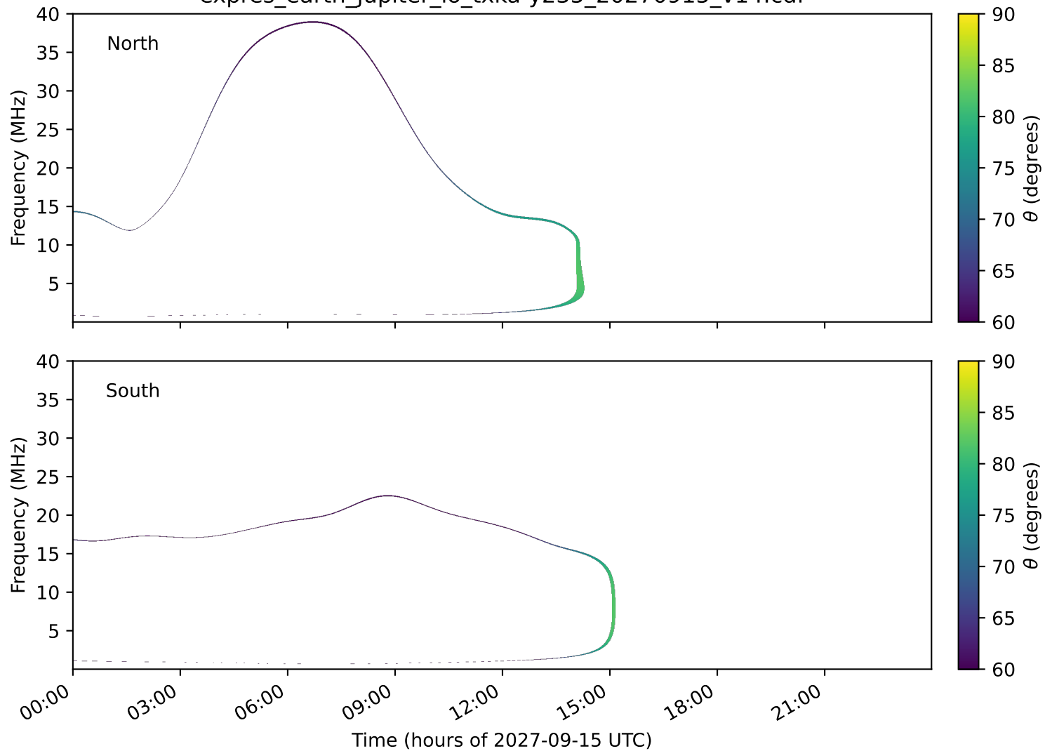
expres_earth_jupiter_io_txka-y235_20270915_v14.cdf
