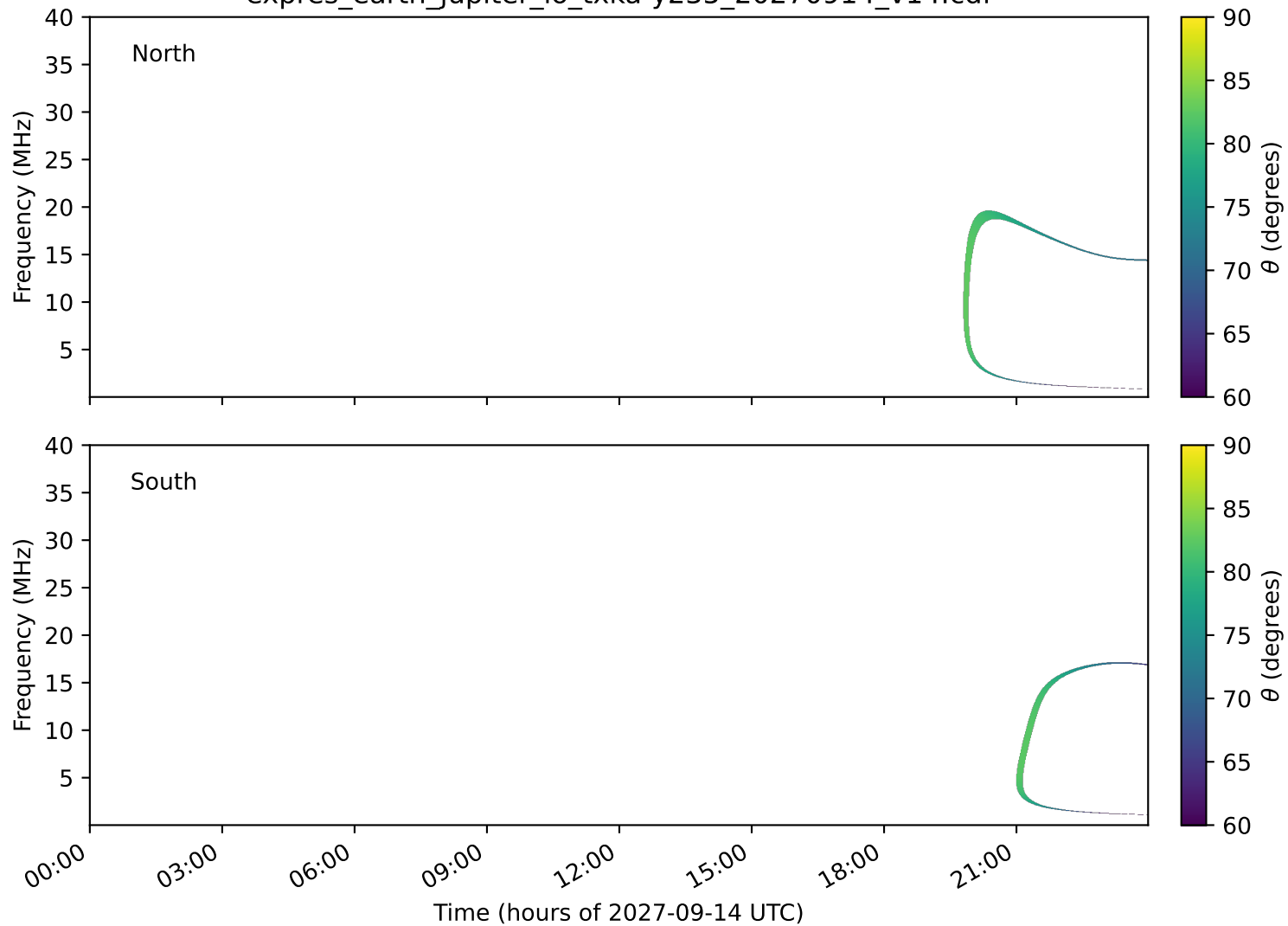
expres_earth_jupiter_io_txka-y235_20270914_v14.cdf
