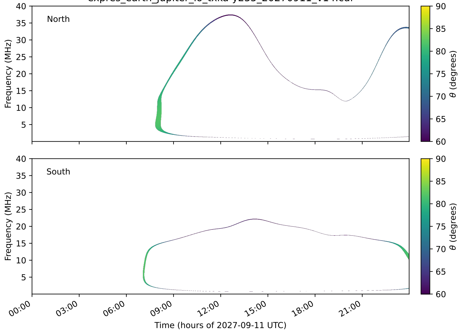
expres_earth_jupiter_io_txka-y235_20270911_v14.cdf
