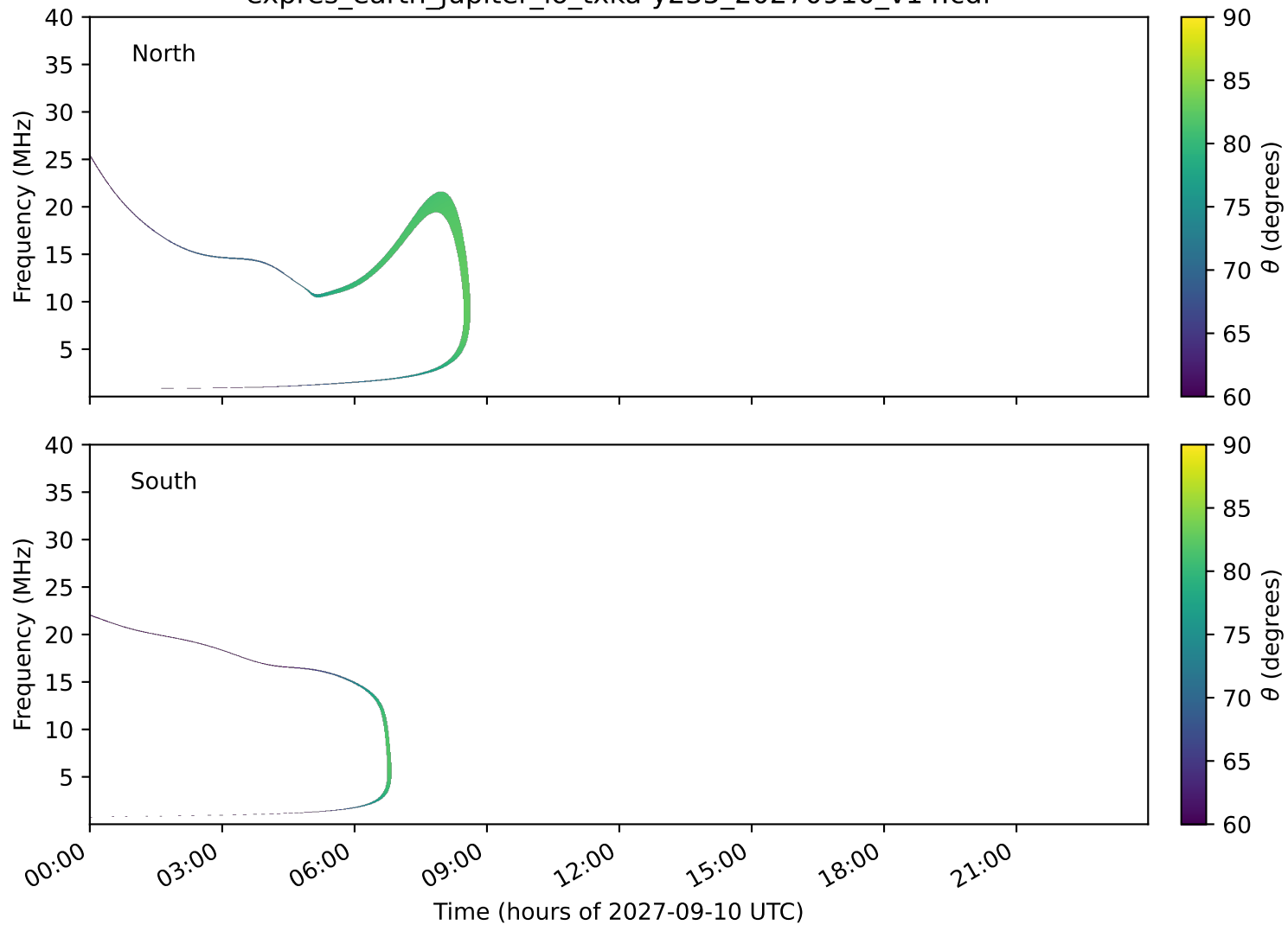
expres_earth_jupiter_io_txka-y235_20270910_v14.cdf
