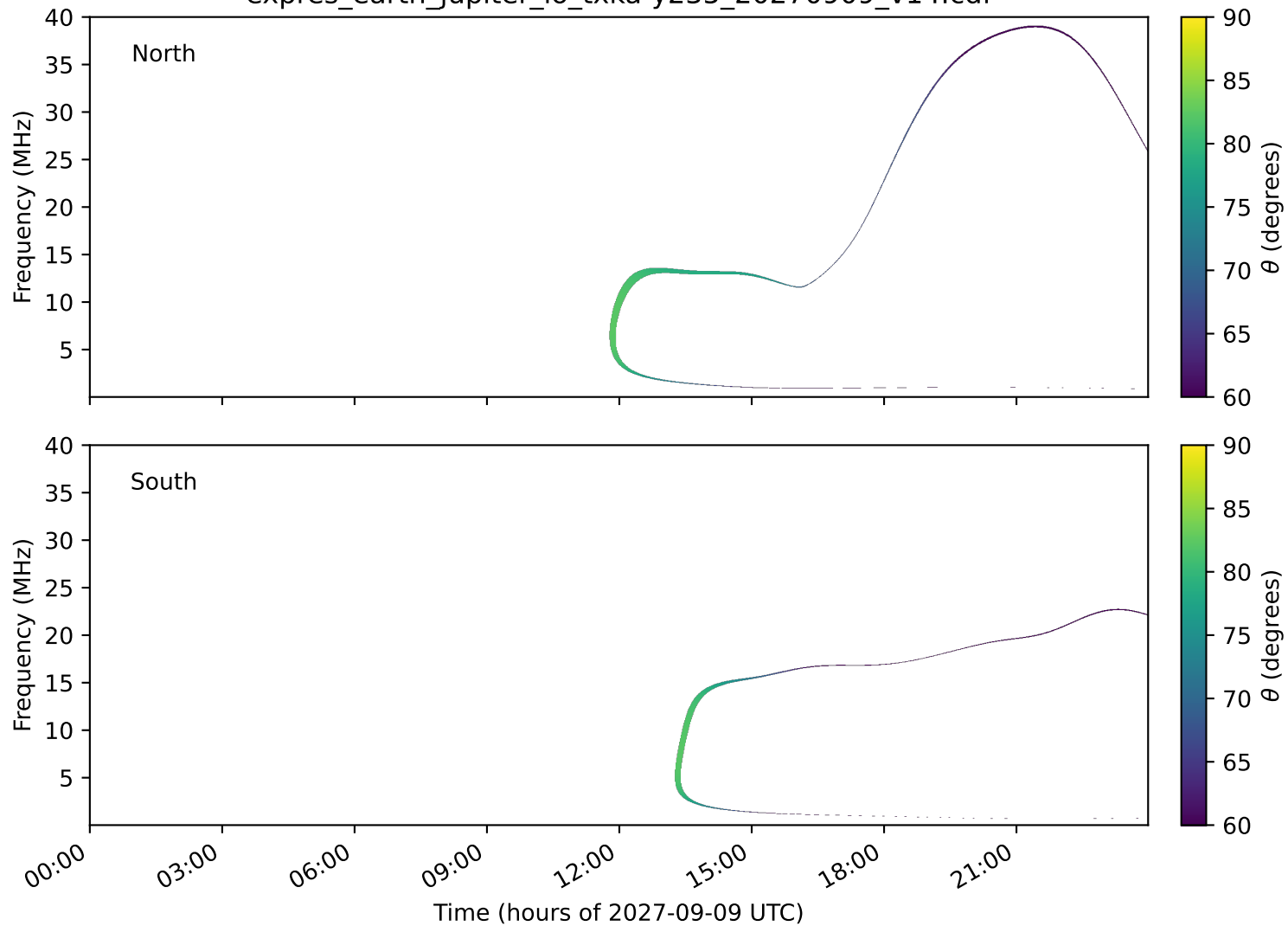
expres_earth_jupiter_io_txka-y235_20270909_v14.cdf
