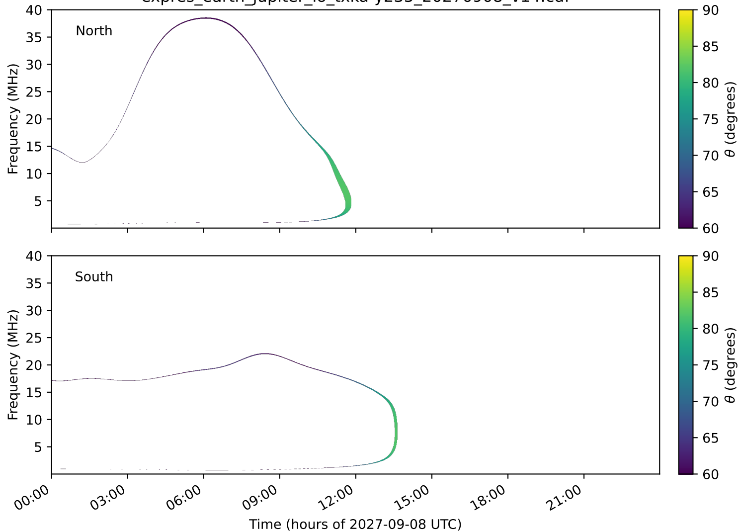
expres_earth_jupiter_io_txka-y235_20270908_v14.cdf
