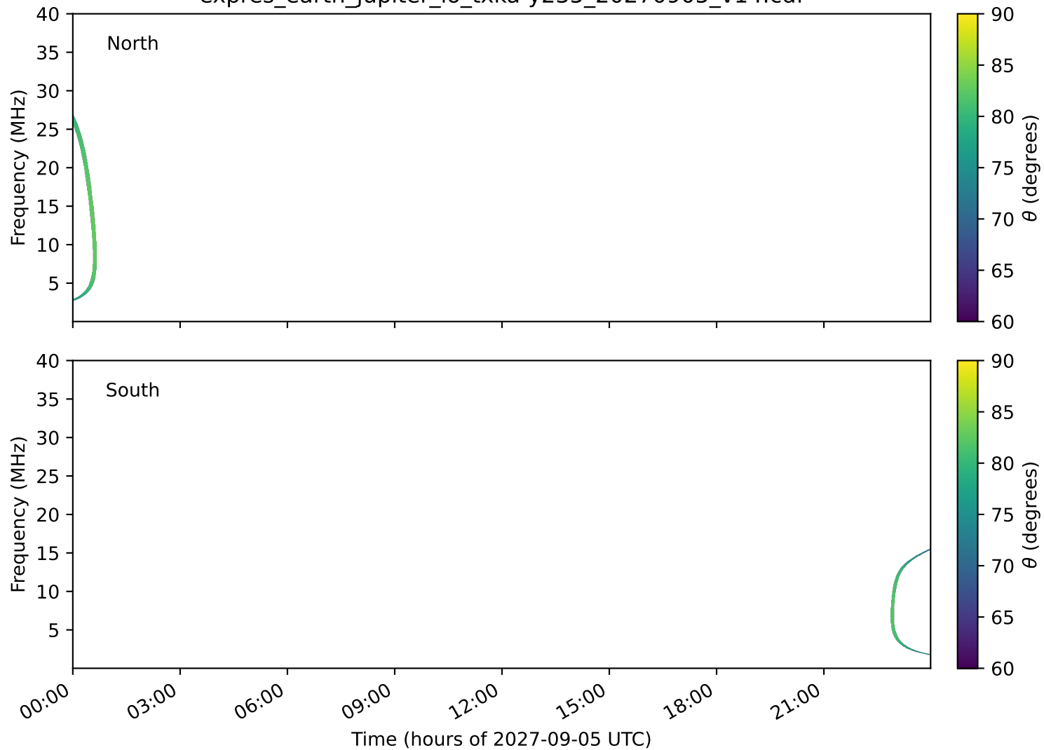
expres_earth_jupiter_io_txka-y235_20270905_v14.cdf
