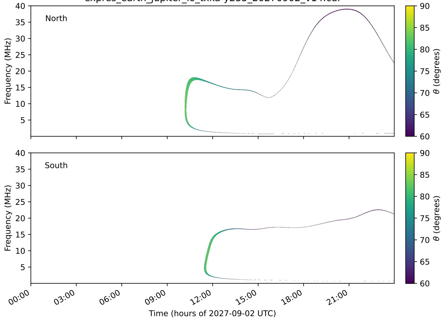
expres_earth_jupiter_io_txka-y235_20270902_v14.cdf
