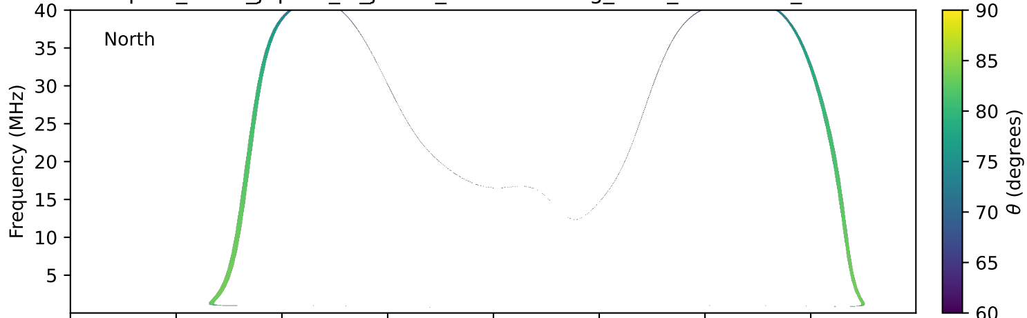
expres_earth_jupiter_io_jrm33_lossc-wid1deg_3kev_20270929_v11.cdf
