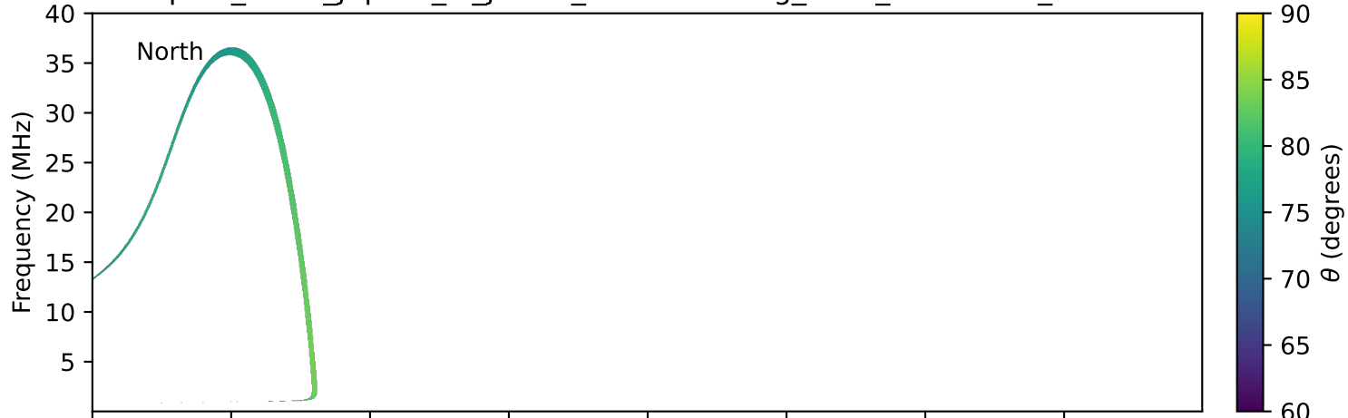
expres_earth_jupiter_io_jrm33_lossc-wid1deg_3kev_20270928_v11.cdf
