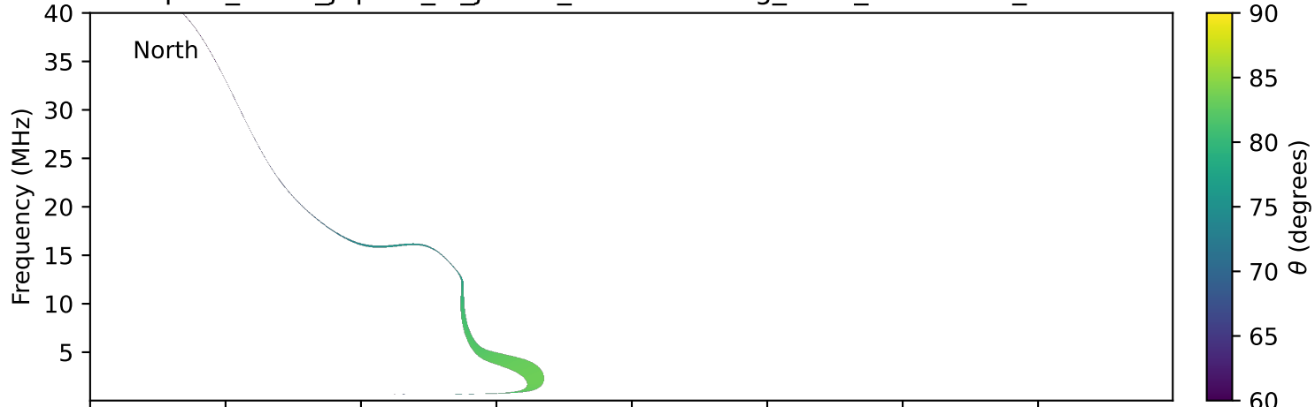
expres_earth_jupiter_io_jrm33_lossc-wid1deg_3kev_20270926_v11.cdf
