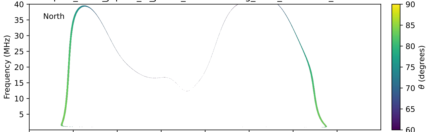
expres_earth_jupiter_io_jrm33_lossc-wid1deg_3kev_20270913_v11.cdf
