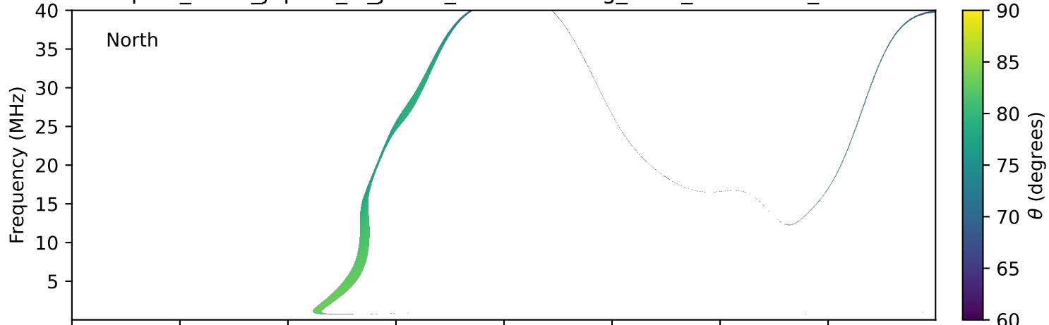
expres_earth_jupiter_io_jrm33_lossc-wid1deg_3kev_20270911_v11.cdf
