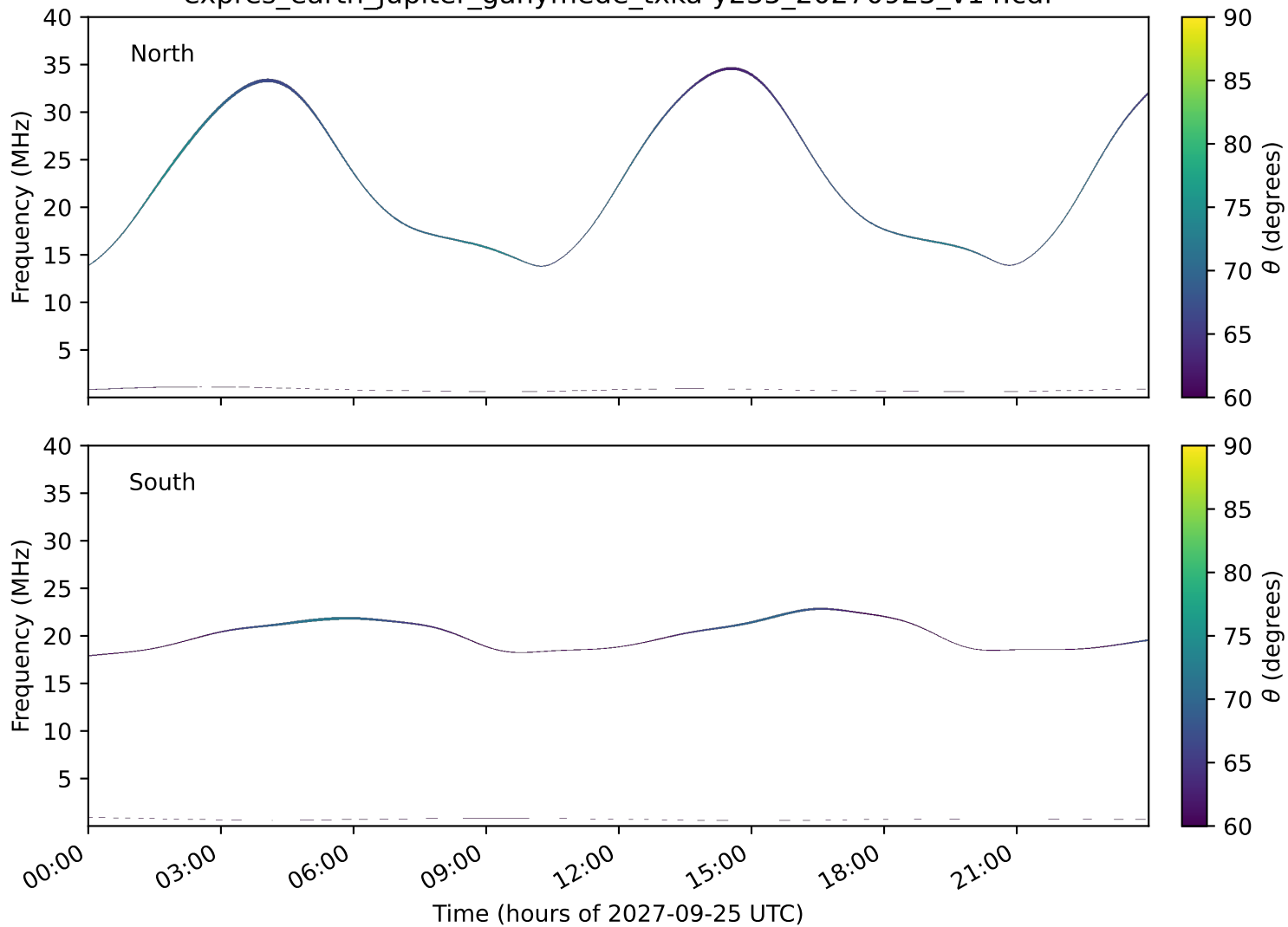
expres_earth_jupiter_ganymede_txka-y235_20270925_v14.cdf
