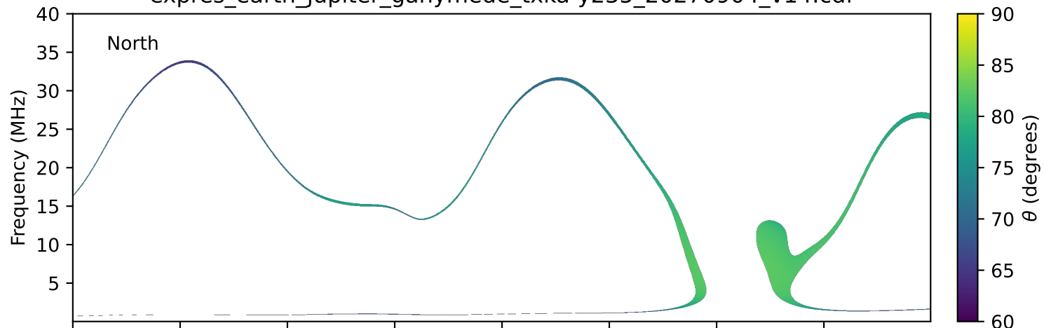
expres_earth_jupiter_ganymede_txka-y235_20270904_v14.cdf
