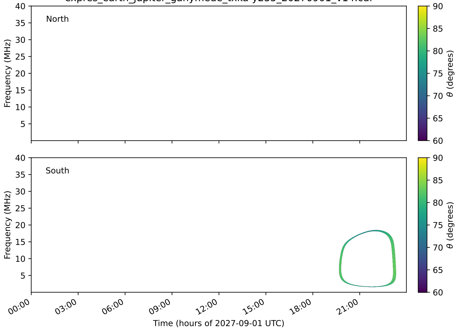
expres_earth_jupiter_ganymede_txka-y235_20270901_v14.cdf
