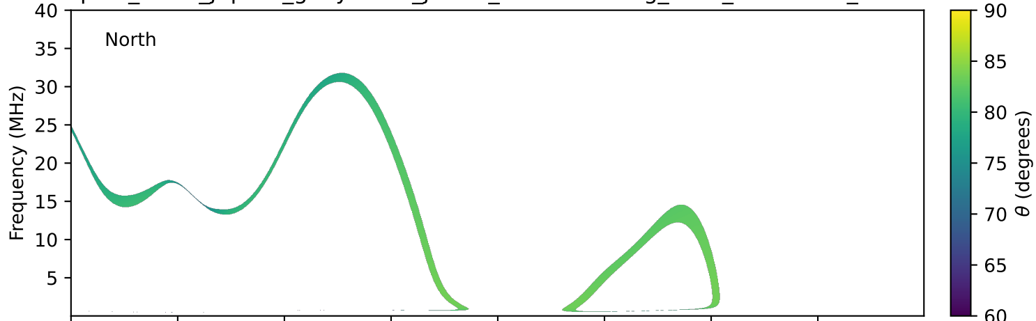
expres_earth_jupiter_ganymede_jrm33_lossc-wid1deg_3kev_20270927_v11.cdf
