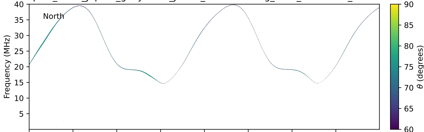
expres_earth_jupiter_ganymede_jrm33_lossc-wid1deg_3kev_20270918_v11.cdf
