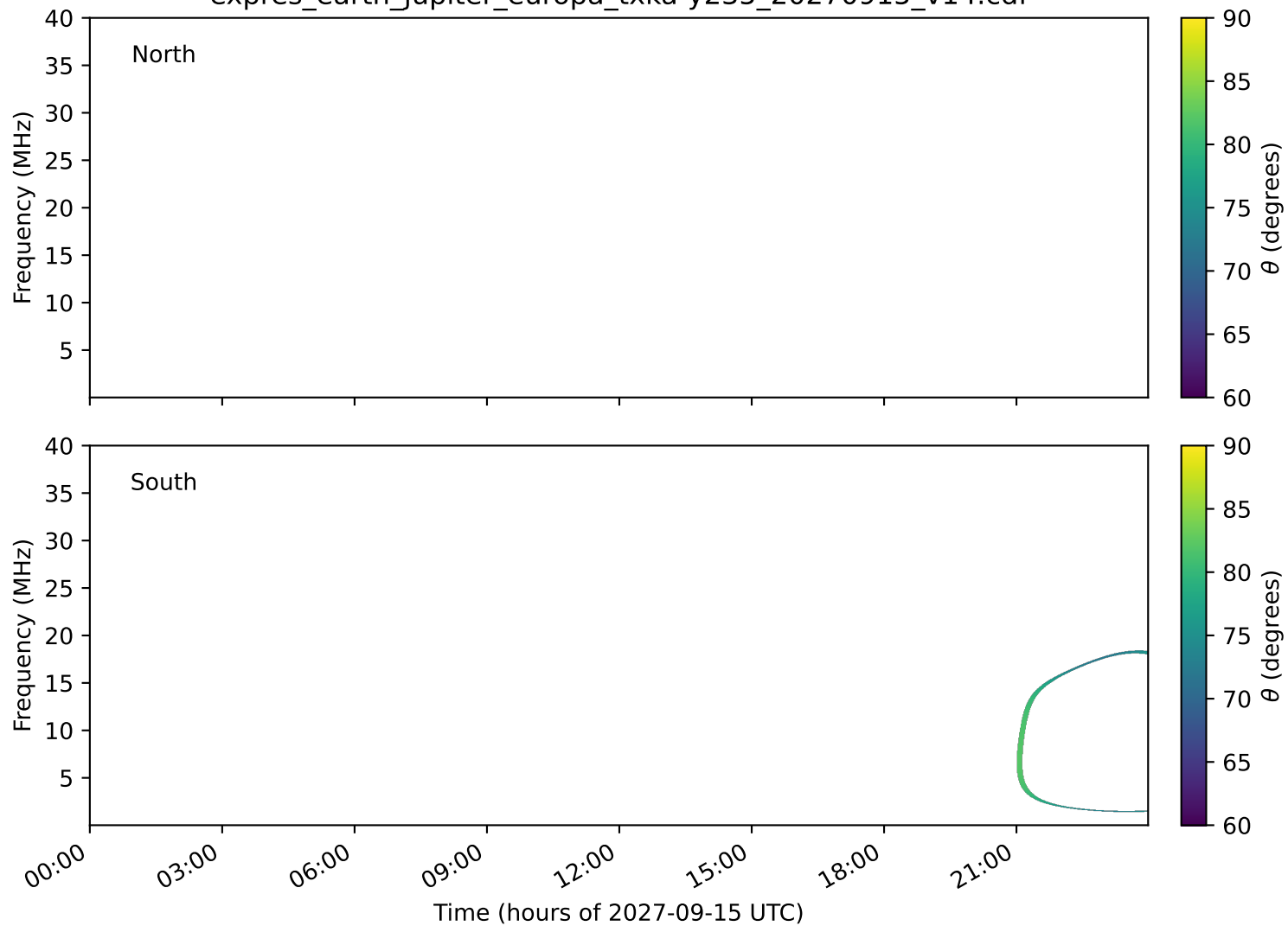
expres_earth_jupiter_europa_txka-y235_20270915_v14.cdf
