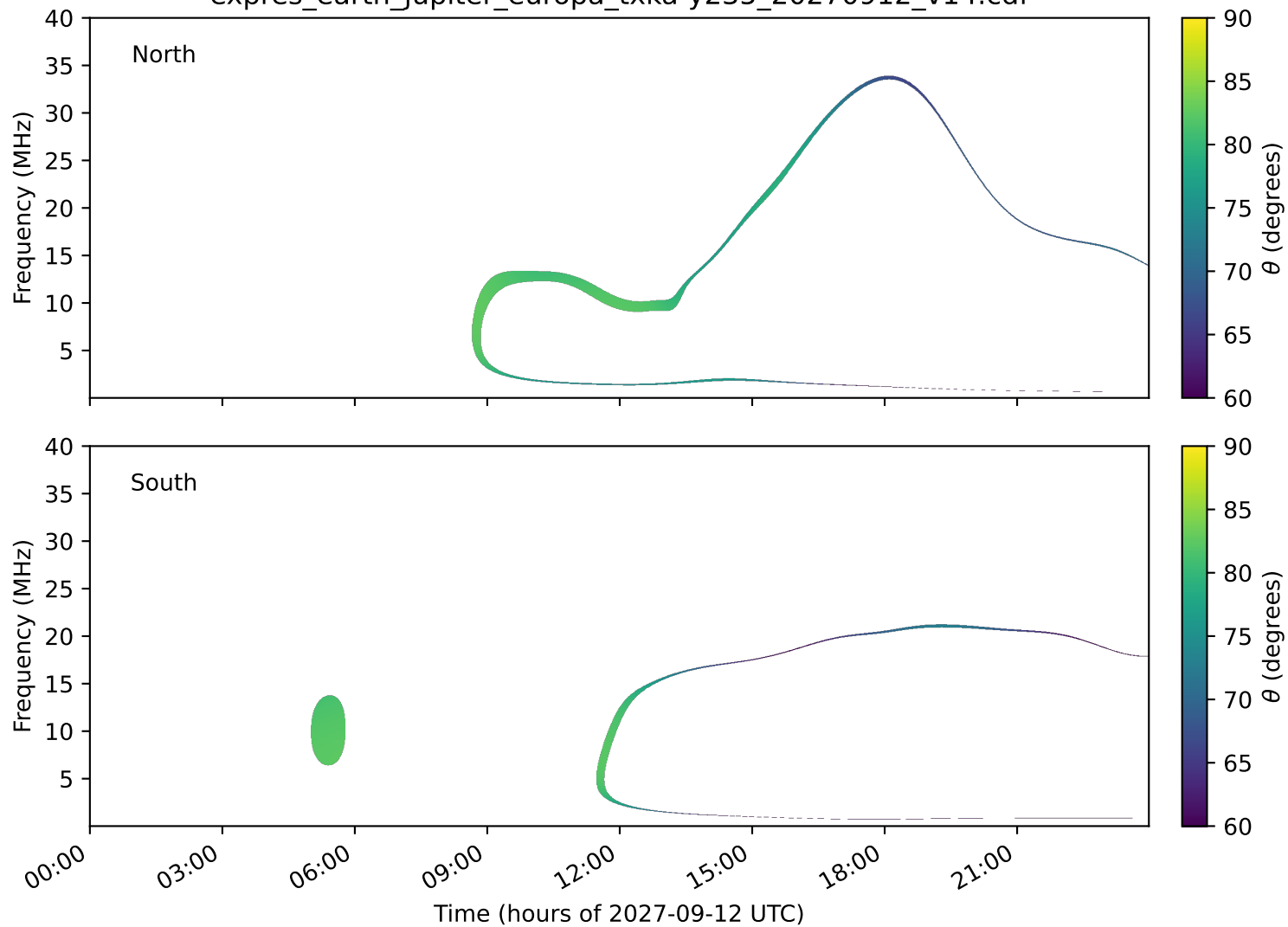
expres_earth_jupiter_europa_txka-y235_20270912_v14.cdf
