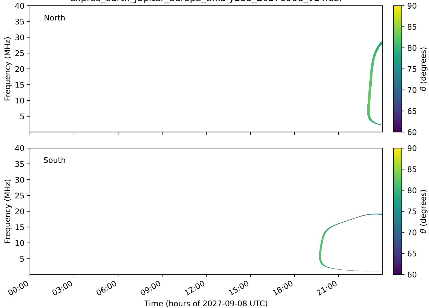
expres_earth_jupiter_europa_txka-y235_20270908_v14.cdf
