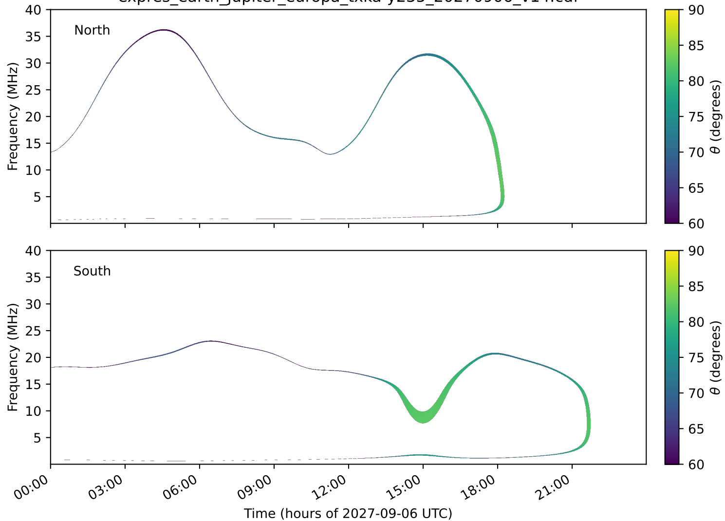
expres_earth_jupiter_europa_txka-y235_20270906_v14.cdf
