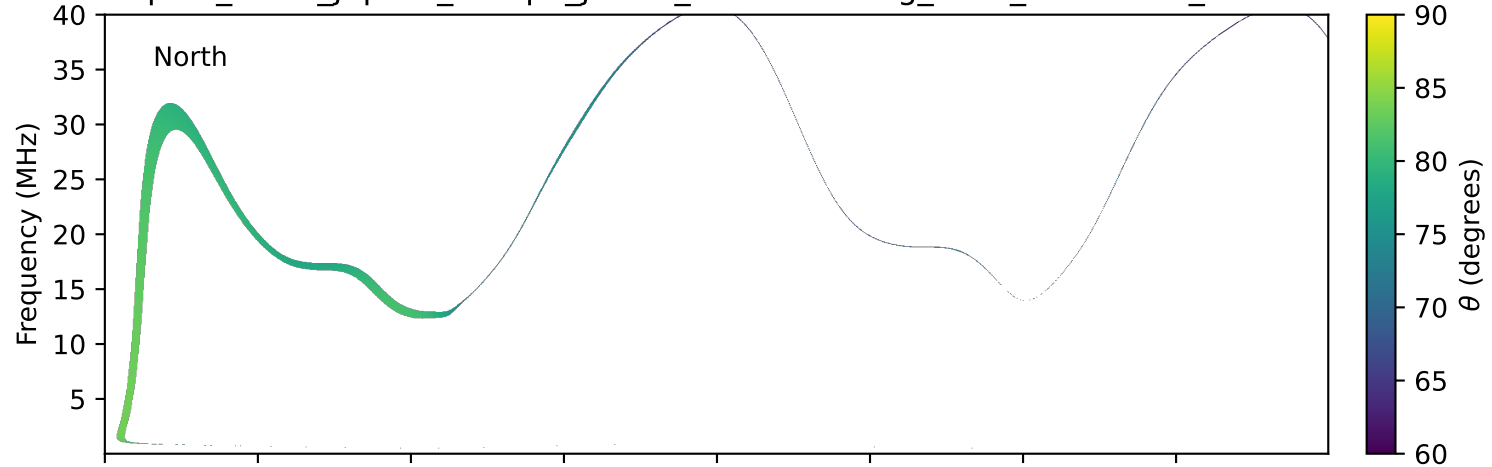
expres_earth_jupiter_europa_jrm33_lossc-wid1deg_3kev_20270916_v11.cdf
