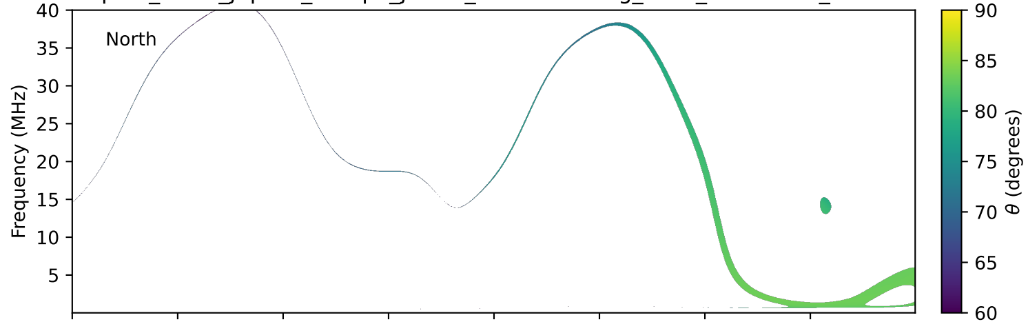
expres_earth_jupiter_europa_jrm33_lossc-wid1deg_3kev_20270906_v11.cdf
