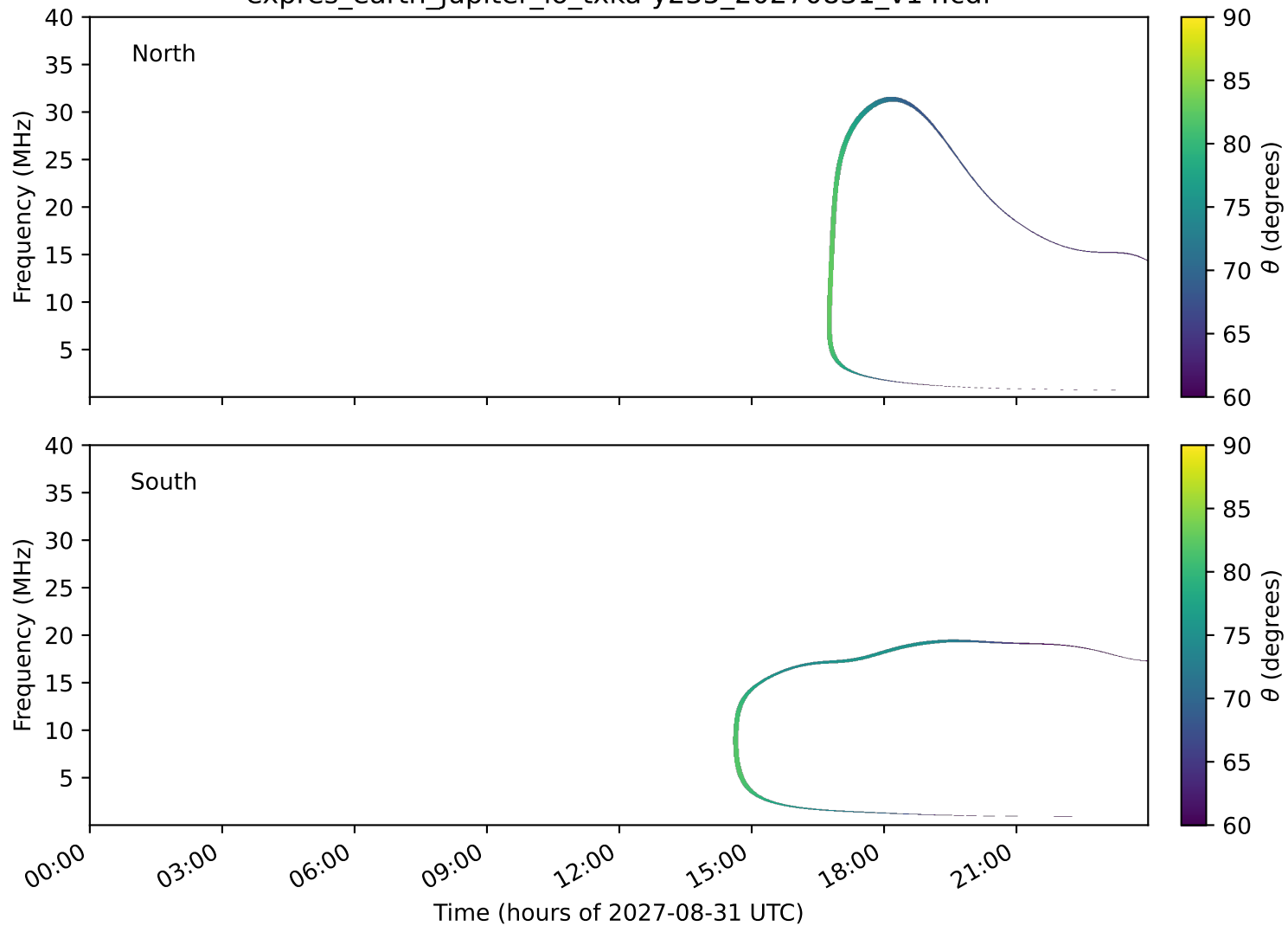
expres_earth_jupiter_io_txka-y235_20270831_v14.cdf
