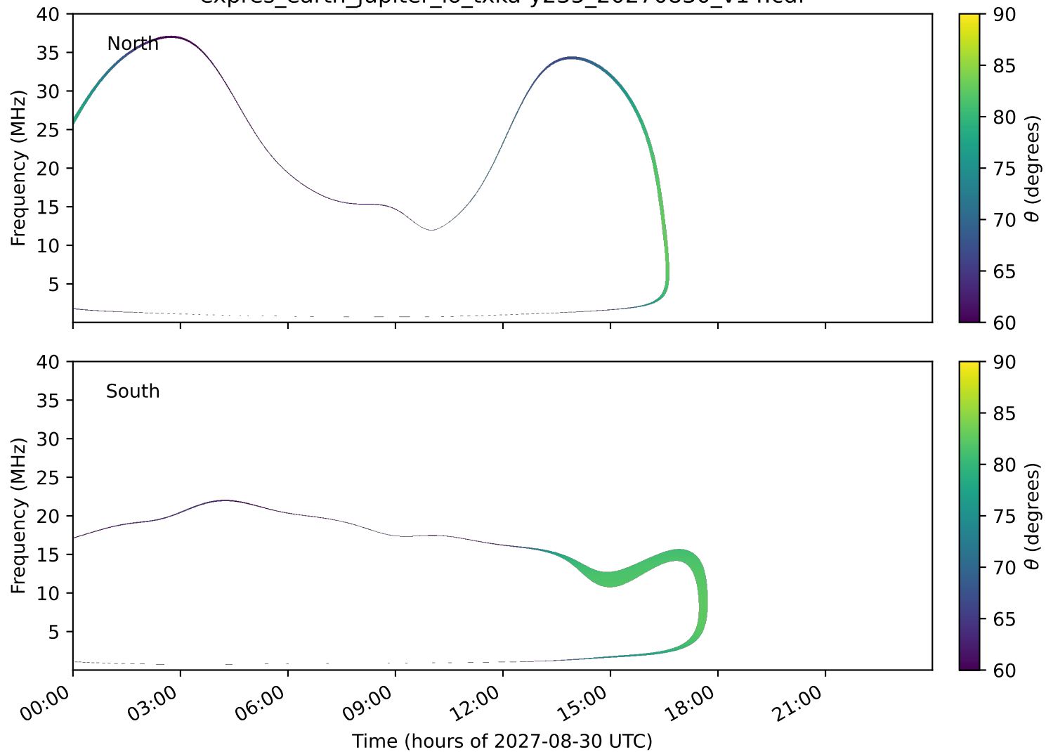
expres_earth_jupiter_io_txka-y235_20270830_v14.cdf
