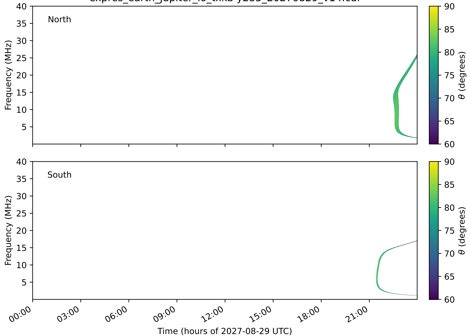
expres_earth_jupiter_io_txka-y235_20270829_v14.cdf
