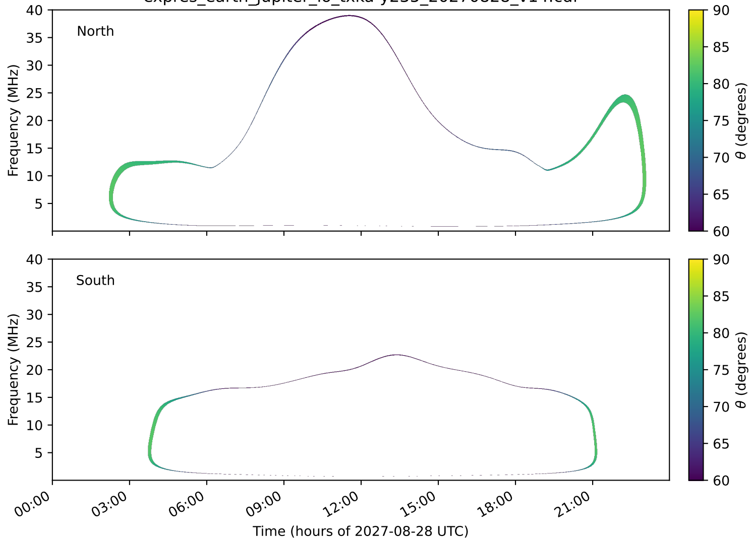
expres_earth_jupiter_io_txka-y235_20270828_v14.cdf
