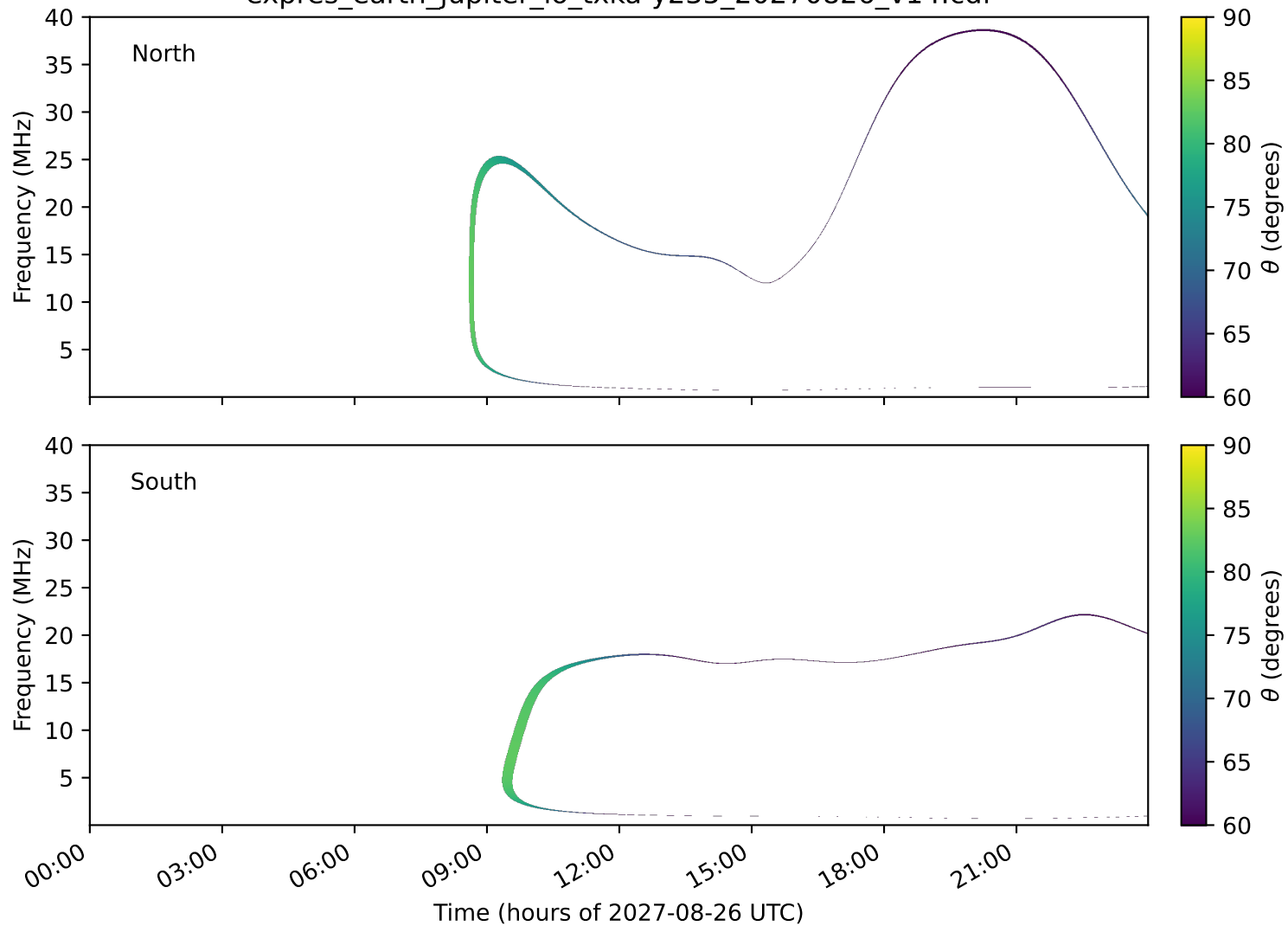
expres_earth_jupiter_io_txka-y235_20270826_v14.cdf
