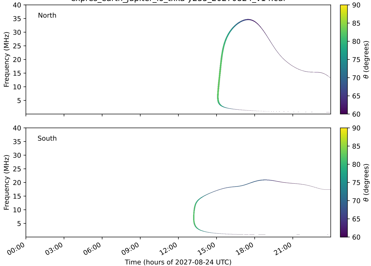
expres_earth_jupiter_io_txka-y235_20270824_v14.cdf
