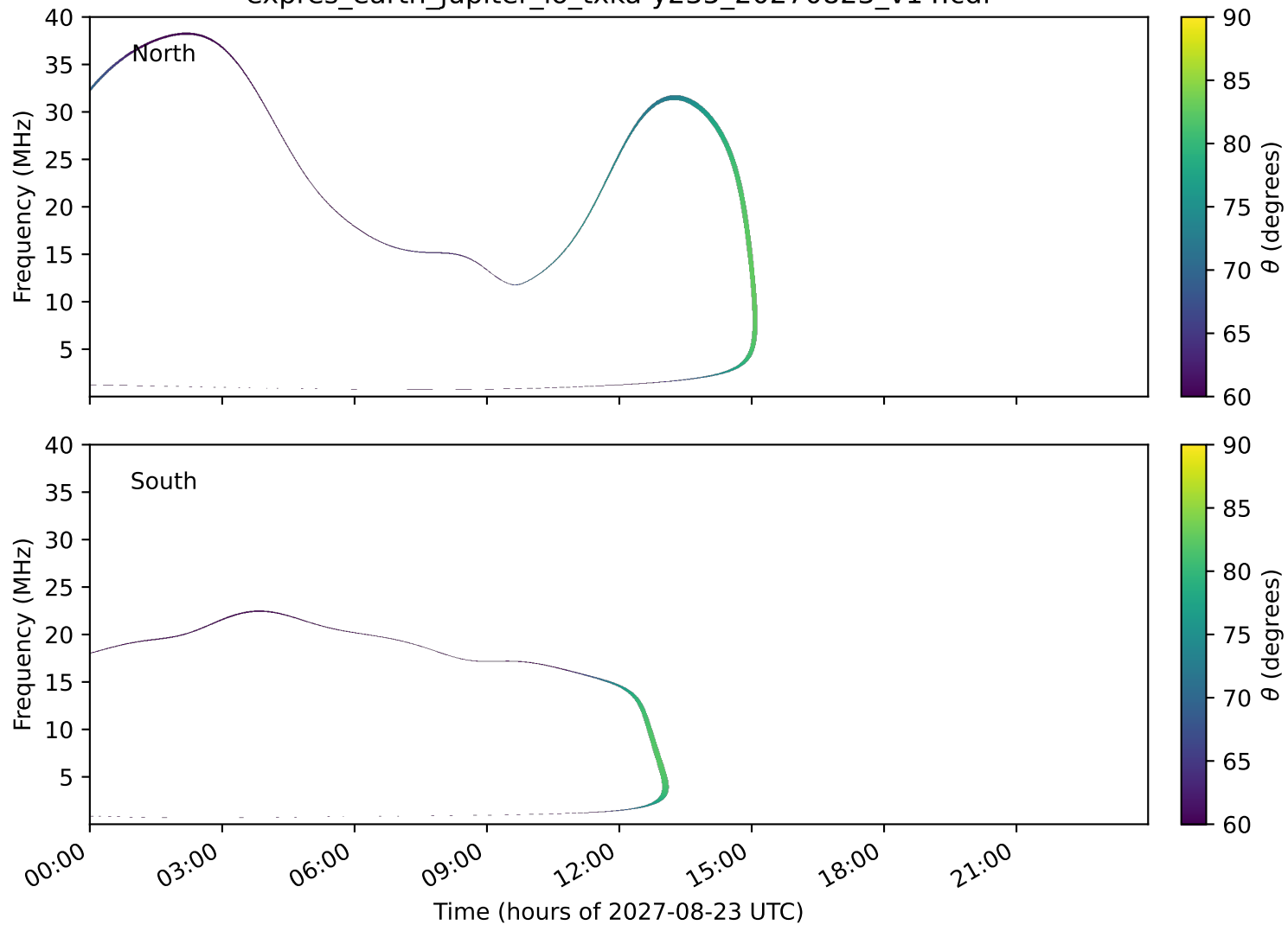
expres_earth_jupiter_io_txka-y235_20270823_v14.cdf
