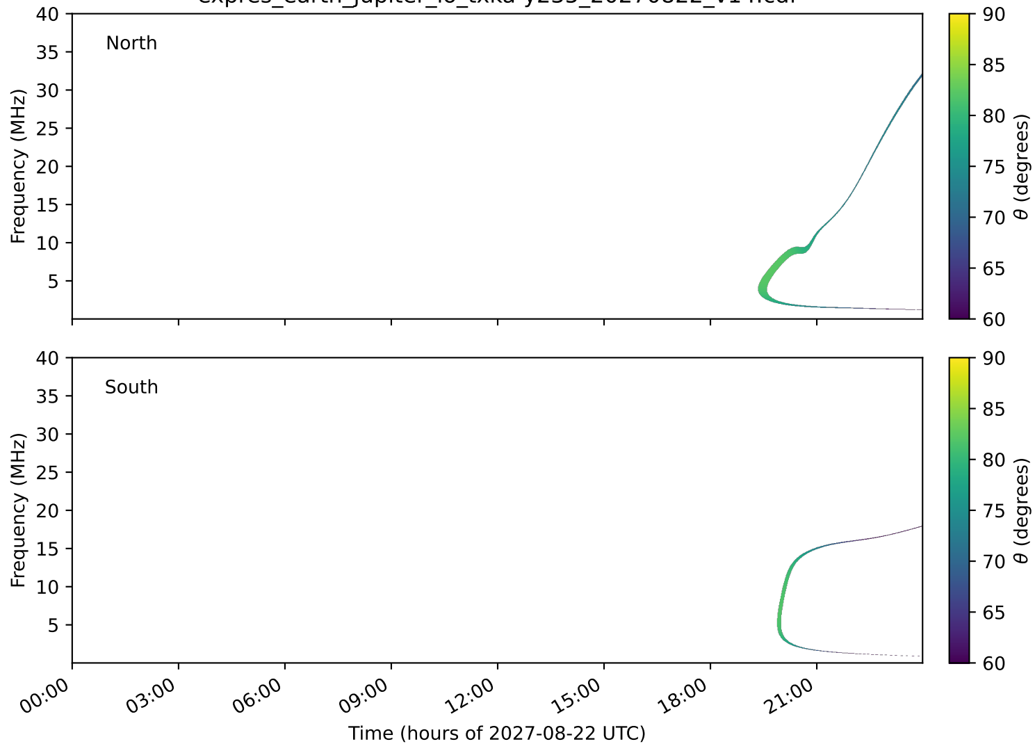
expres_earth_jupiter_io_txka-y235_20270822_v14.cdf
