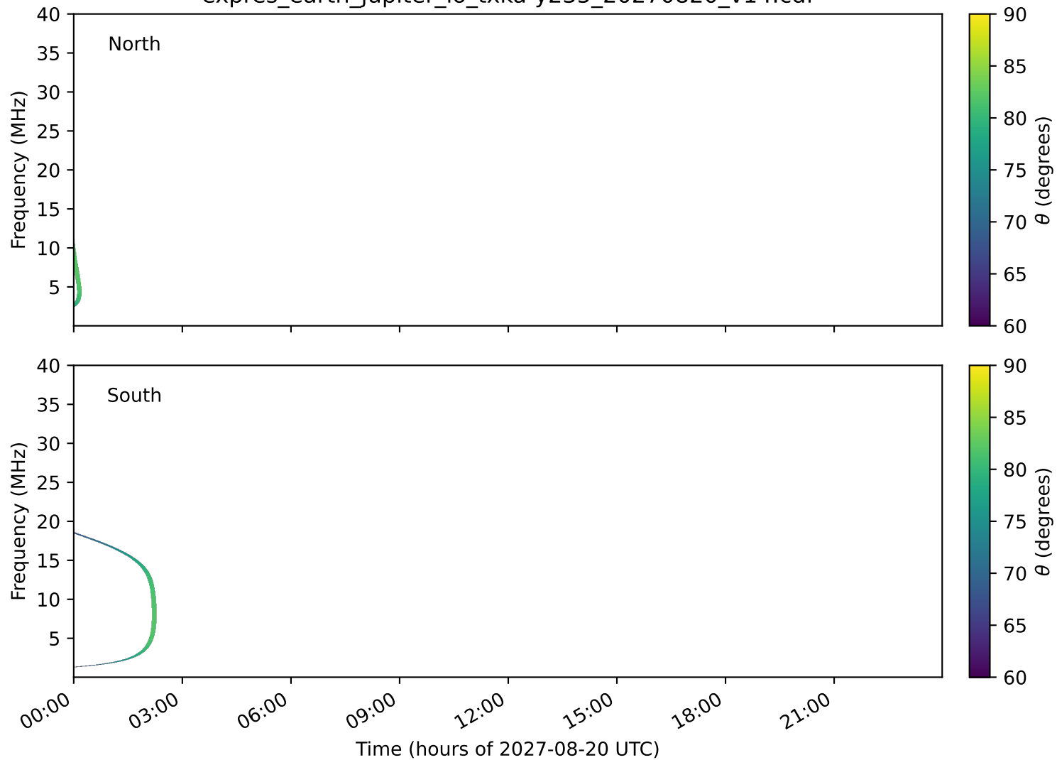
expres_earth_jupiter_io_txka-y235_20270820_v14.cdf
