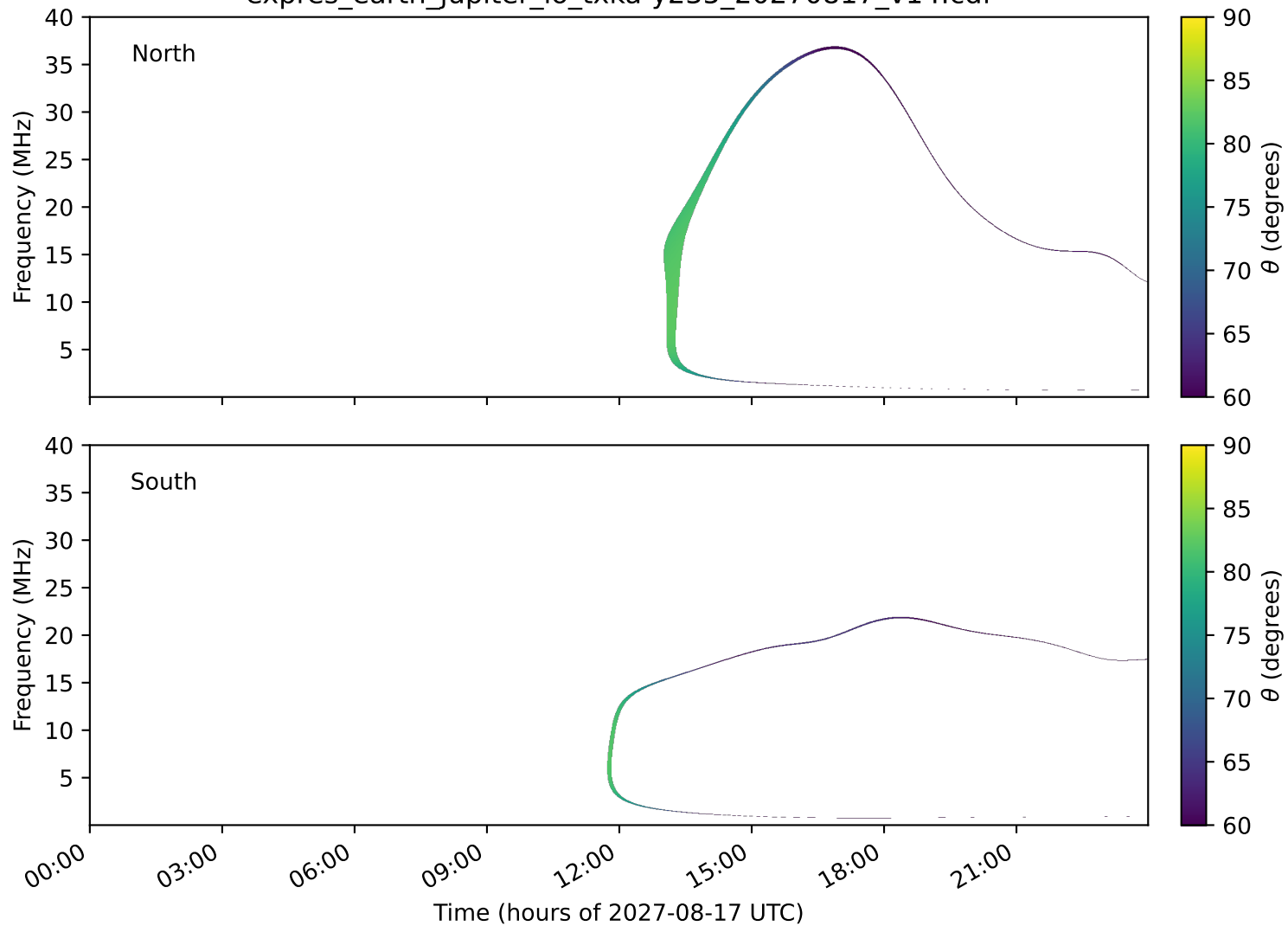
expres_earth_jupiter_io_txka-y235_20270817_v14.cdf
