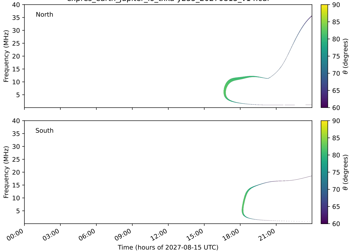
expres_earth_jupiter_io_txka-y235_20270815_v14.cdf
