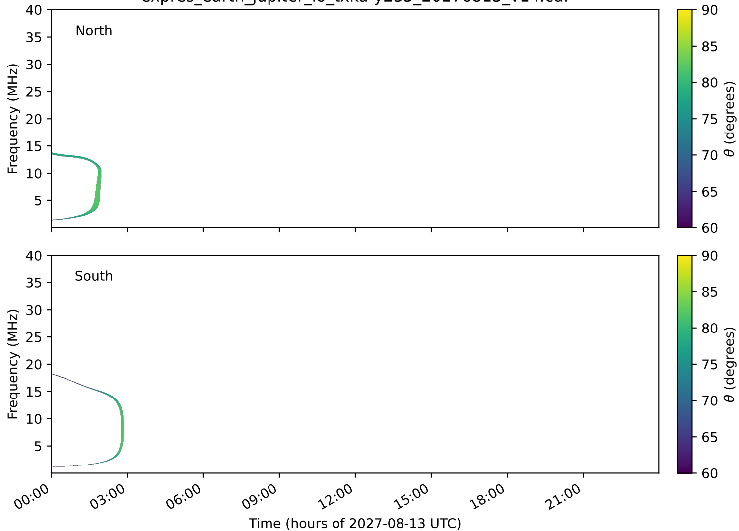
expres_earth_jupiter_io_txka-y235_20270813_v14.cdf
