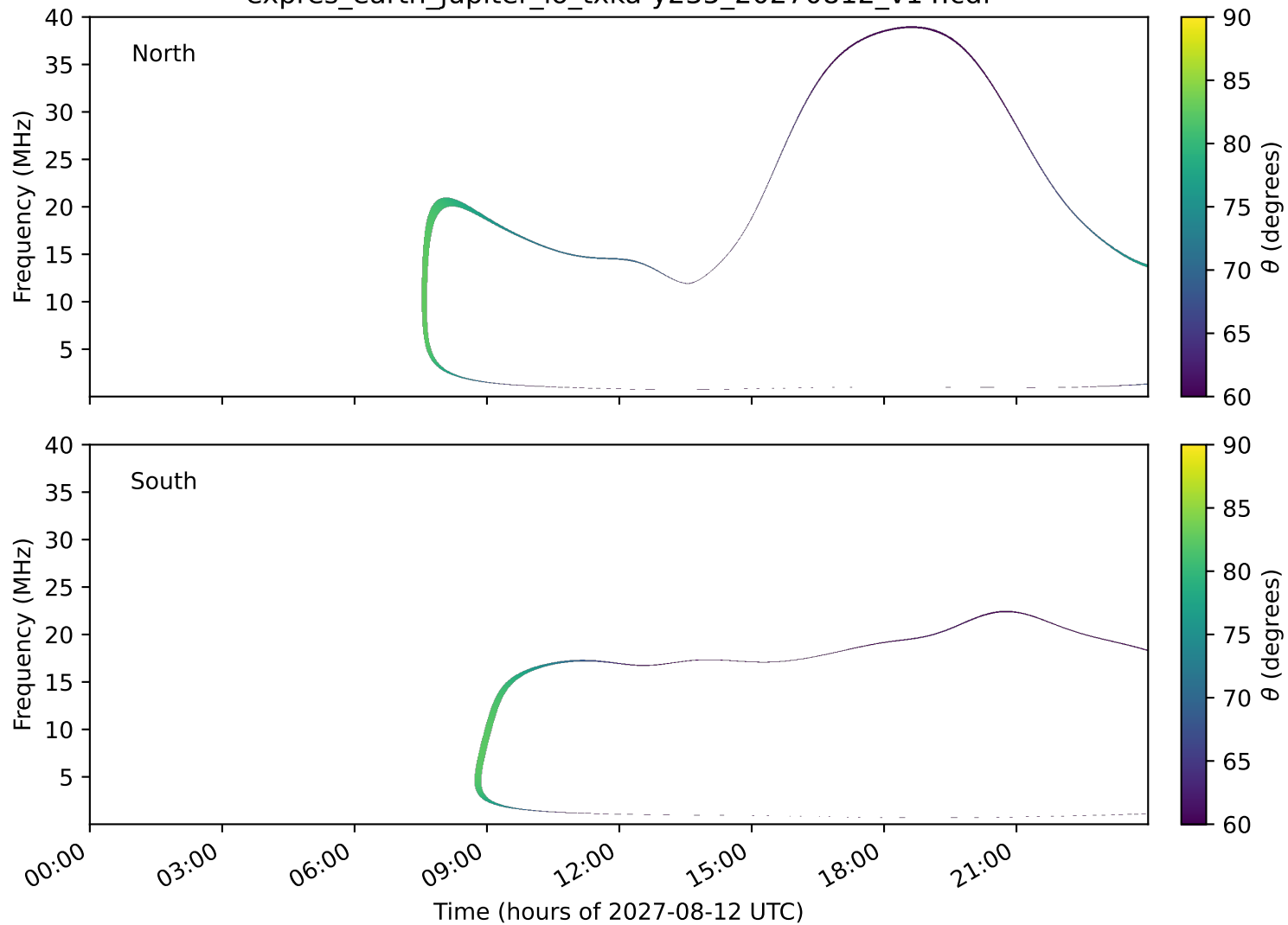
expres_earth_jupiter_io_txka-y235_20270812_v14.cdf
