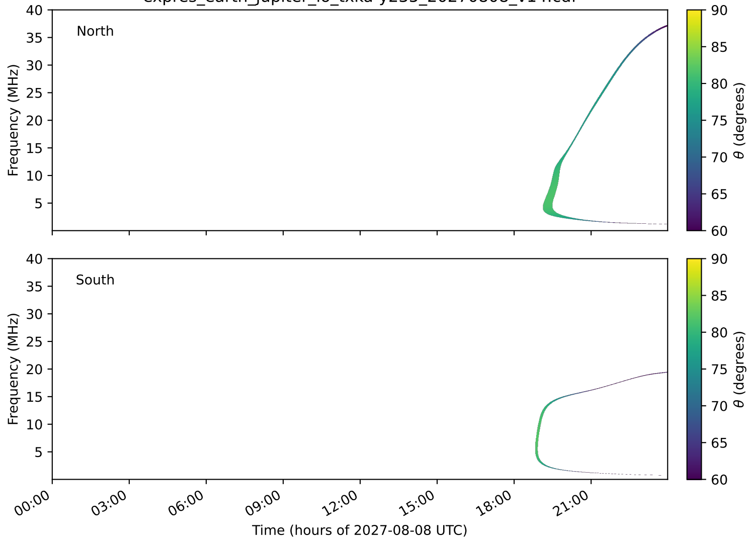
expres_earth_jupiter_io_txka-y235_20270808_v14.cdf
