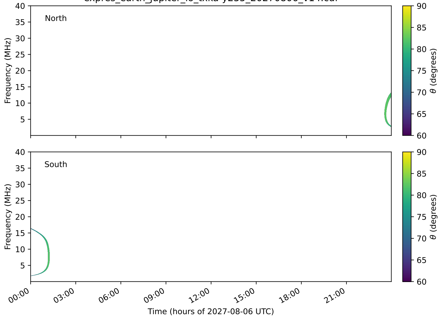
expres_earth_jupiter_io_txka-y235_20270806_v14.cdf
