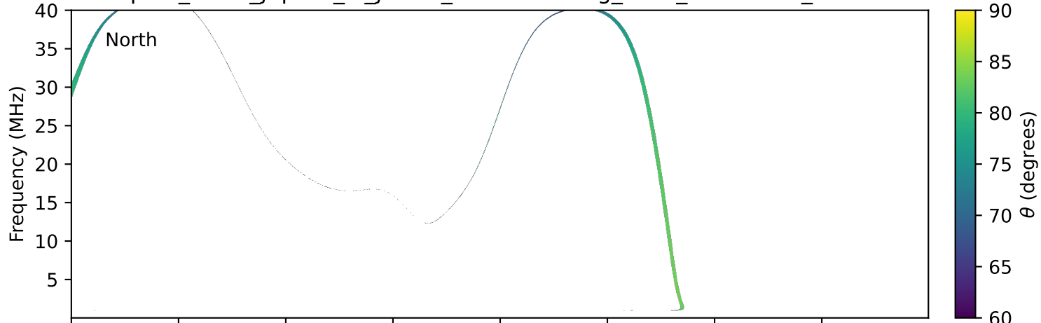
expres_earth_jupiter_io_jrm33_lossc-wid1deg_3kev_20270830_v11.cdf
