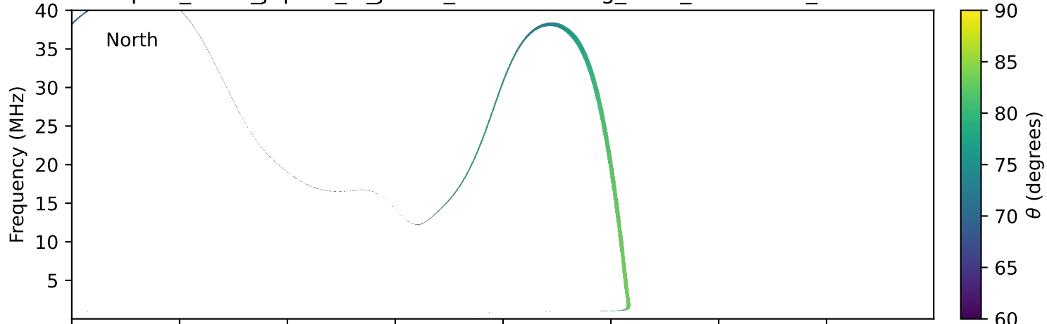
expres_earth_jupiter_io_jrm33_lossc-wid1deg_3kev_20270823_v11.cdf
