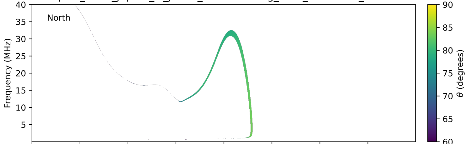
expres_earth_jupiter_io_jrm33_lossc-wid1deg_3kev_20270816_v11.cdf
