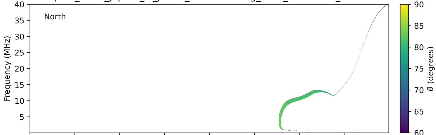
expres_earth_jupiter_io_jrm33_lossc-wid1deg_3kev_20270815_v11.cdf
