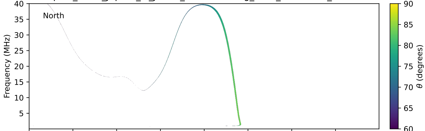
expres_earth_jupiter_io_jrm33_lossc-wid1deg_3kev_20270809_v11.cdf
