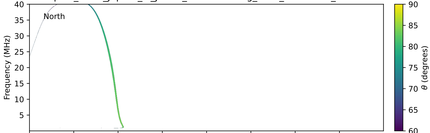
expres_earth_jupiter_io_jrm33_lossc-wid1deg_3kev_20270804_v11.cdf
