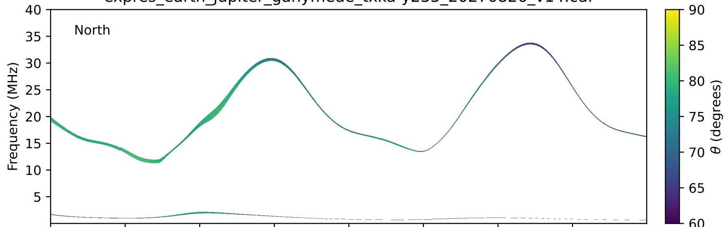
expres_earth_jupiter_ganymede_txka-y235_20270826_v14.cdf
