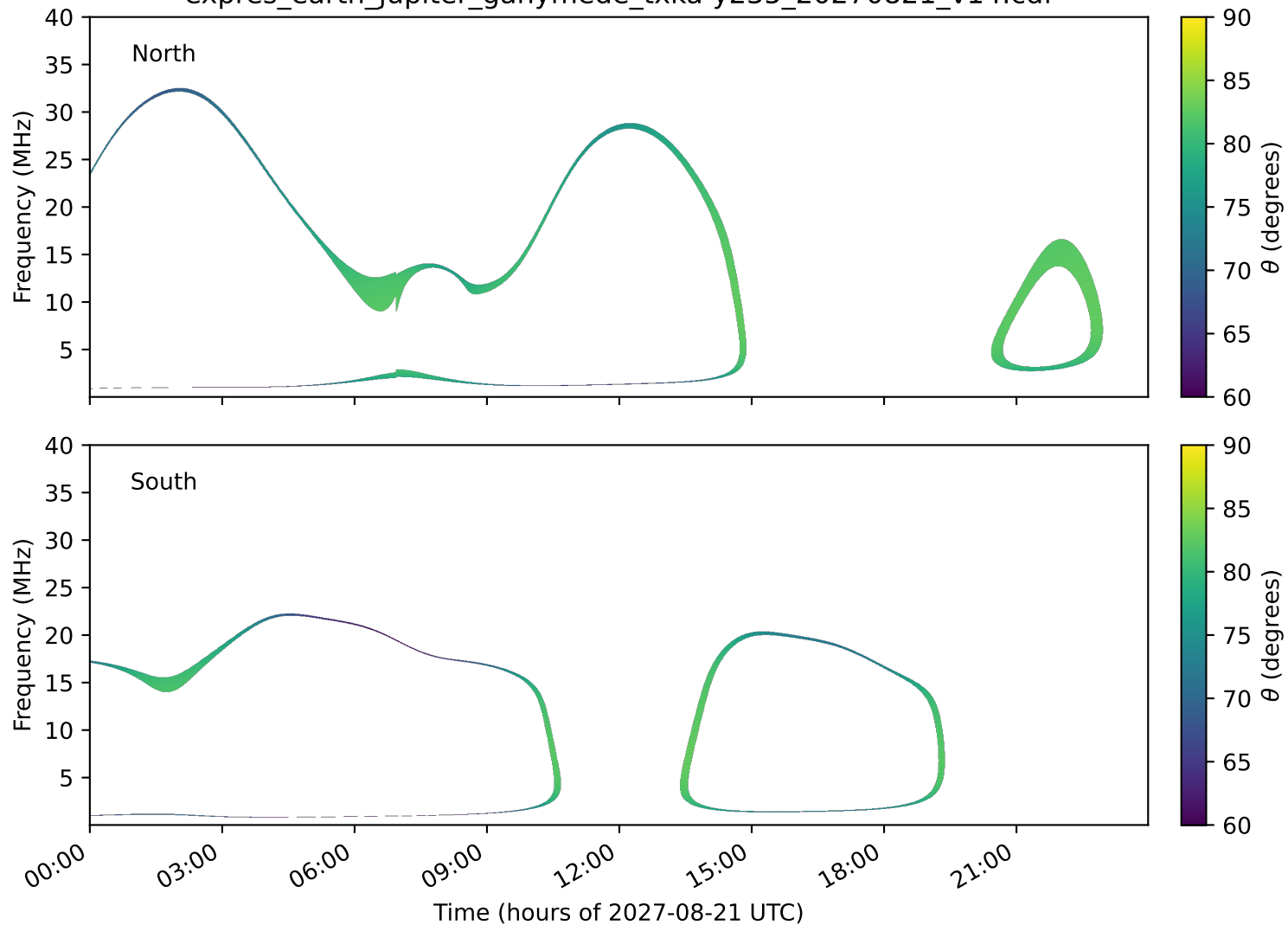
expres_earth_jupiter_ganymede_txka-y235_20270821_v14.cdf
