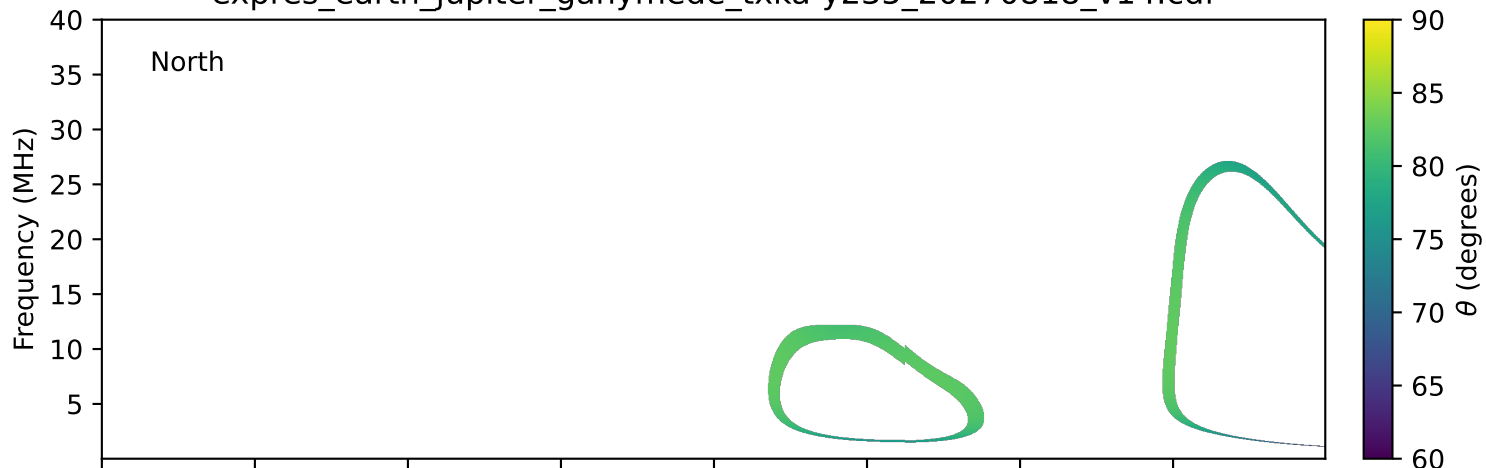
expres_earth_jupiter_ganymede_txka-y235_20270818_v14.cdf
