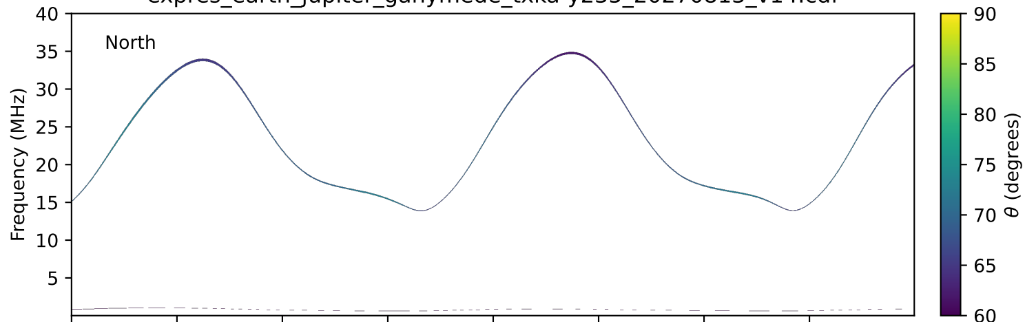
expres_earth_jupiter_ganymede_txka-y235_20270813_v14.cdf
